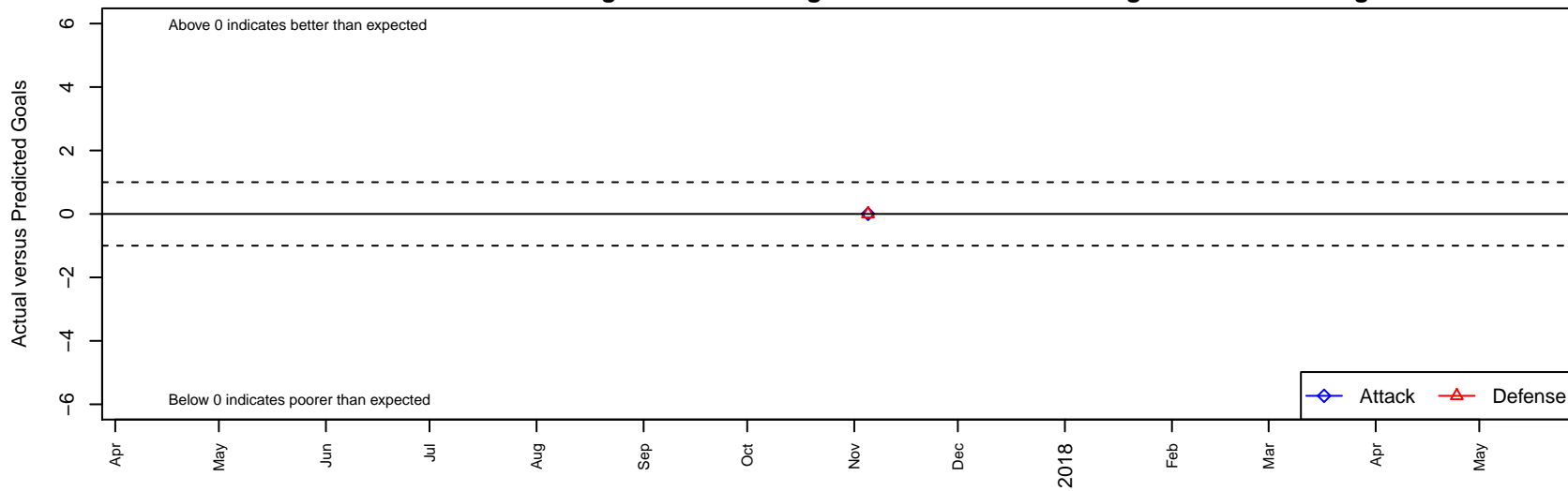
Ballistic United SC USSDA B04 Dots are actual minus expected GF (blue circles) and GA (red triangles). Blue line is smoothed change in attack strength. Red is smoothed change in defense strength.
